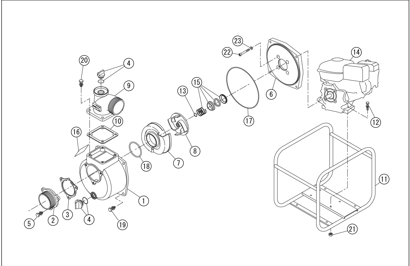
DWG No.011939823 MODEL : SEH-50X FORM : SEH-50X-BAJ-5
