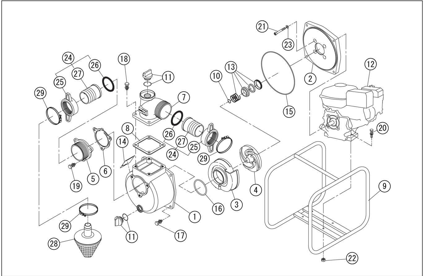
DWG No.066850305 MODEL : SEH-50X FORM : SEH-50X-BCS-2
