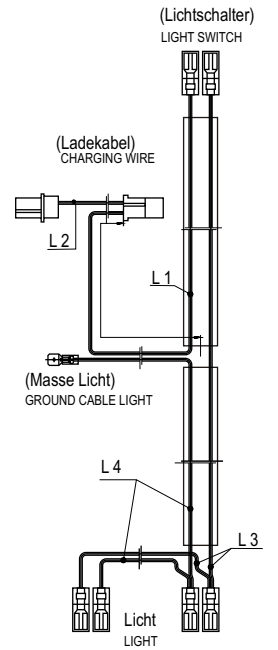
Schaltplan Licht CONNECTION DIAGRAM LIGHT
