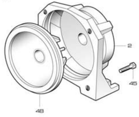
KM 75-100 supporto alluminio aluminium motor bracket
