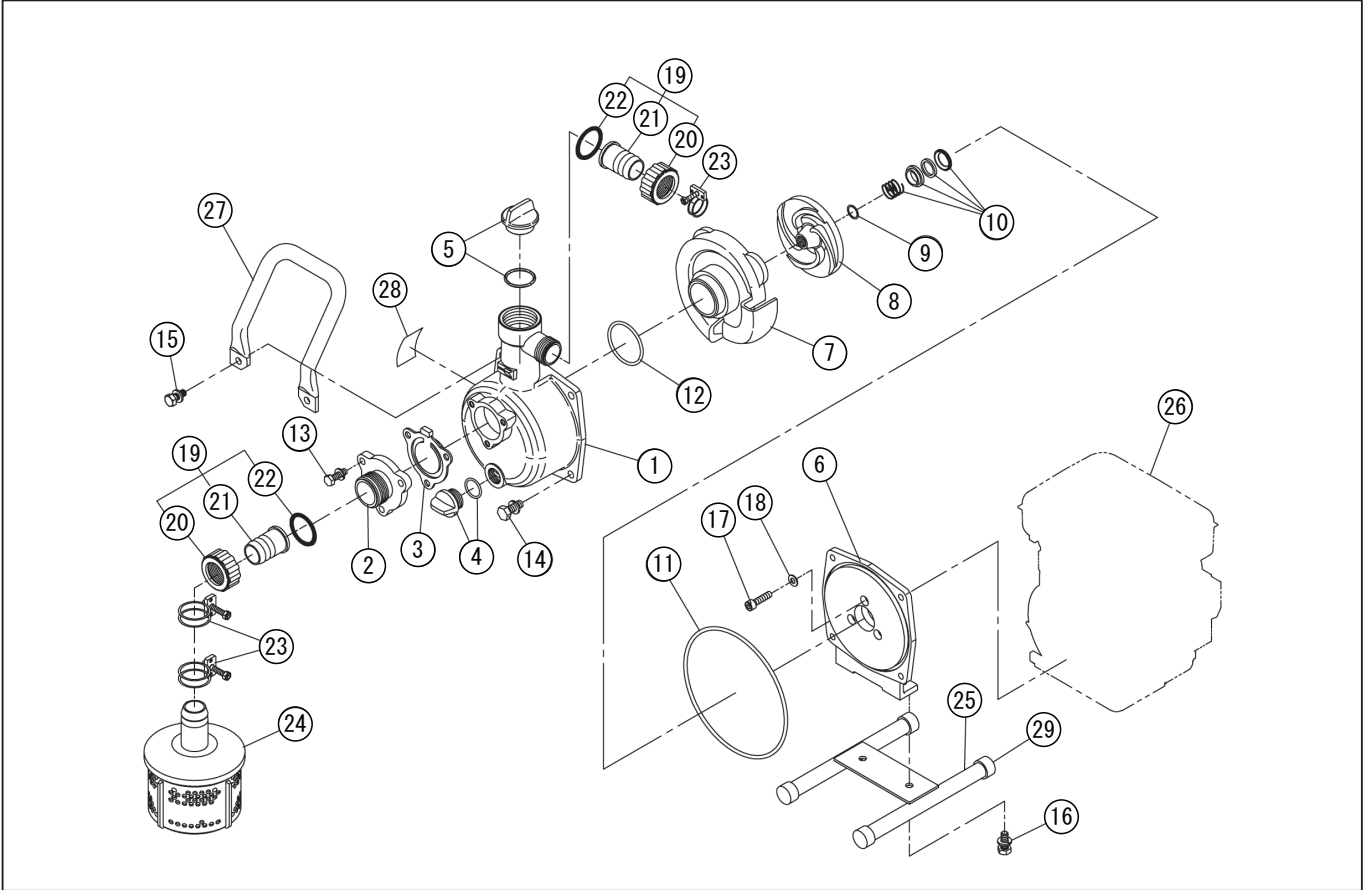
DWG No.012863607 MODELE:SEM-25L FORM:SEM-25L-BAA-3
