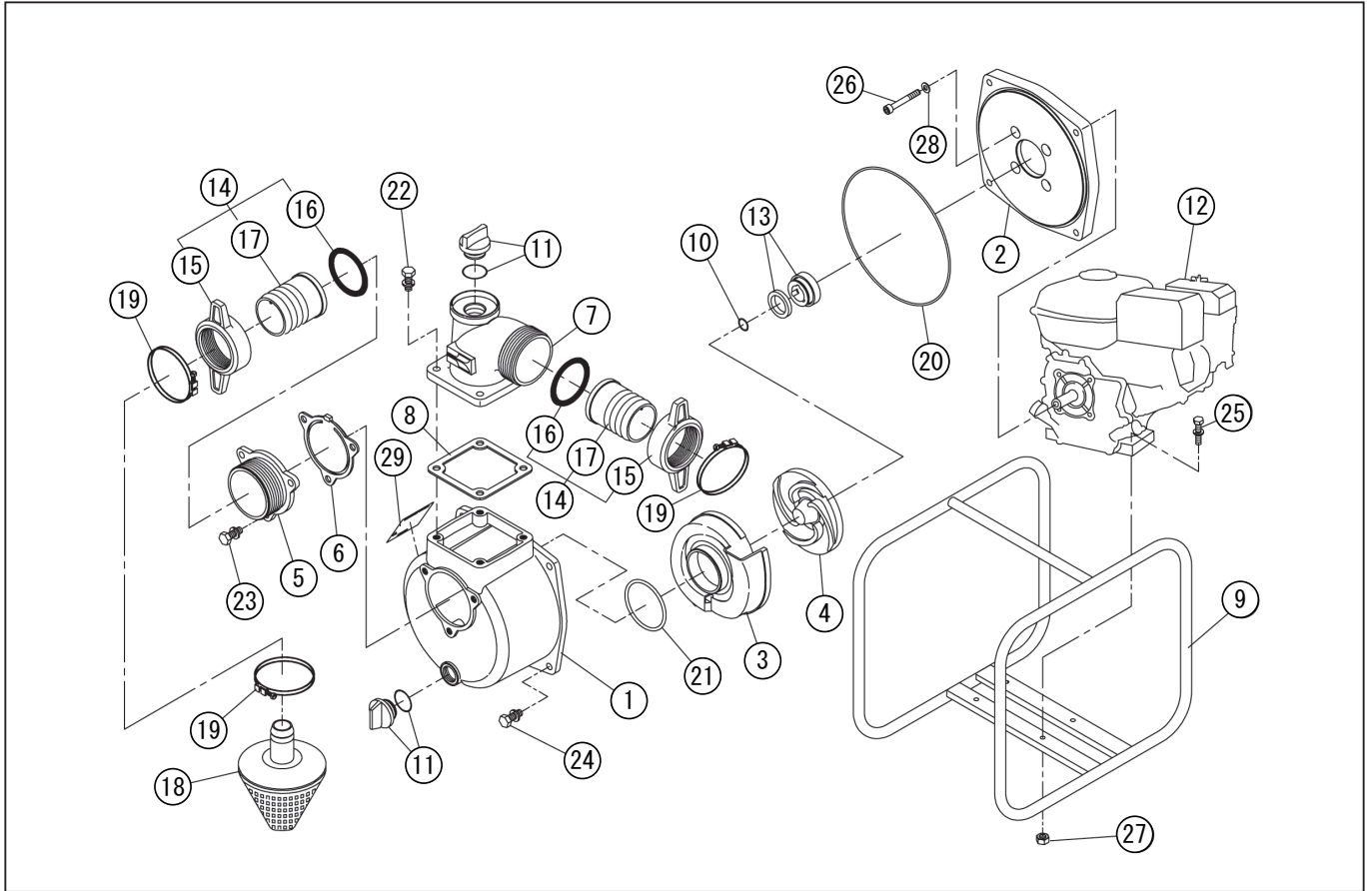
DWG No.066852009 MODEL : SEH-50XK FORM : SEH-50X-BCN-2
