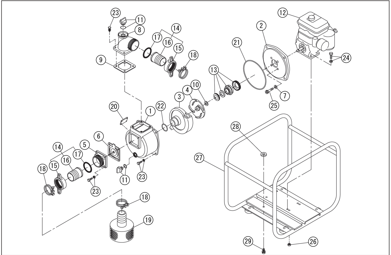
DWG No.012855607 MODEL : SEH-100X FORM : SEH-100X-BAA-1
