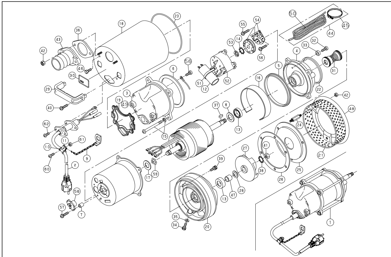
DWG No.043854009 MODEL:PB-55022 FORM:PB-55022-BAD-2
