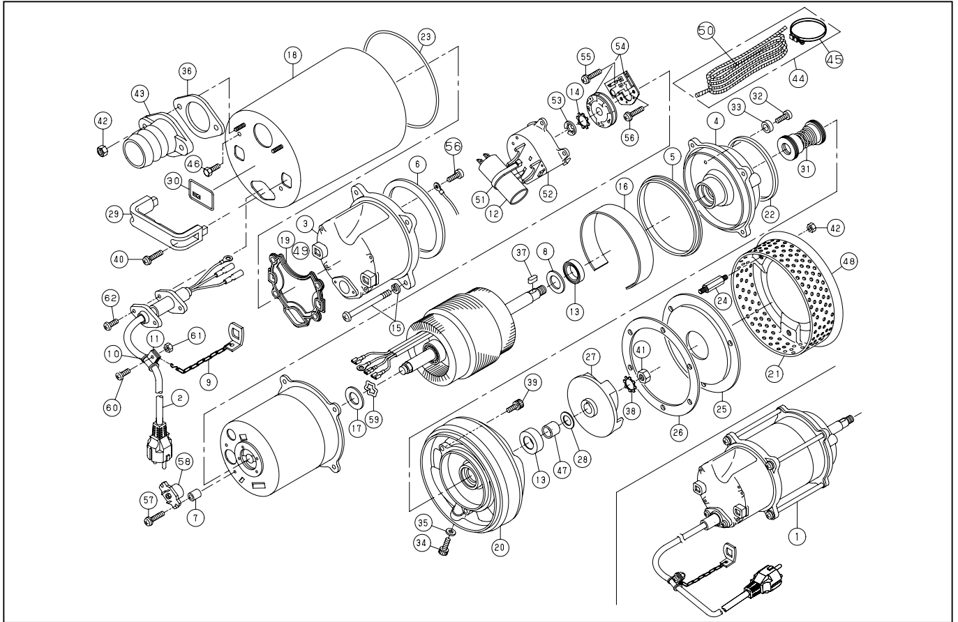
DWG No.043854009 MODEL:PB-55022 FORM:PB-55022-BAD-2
